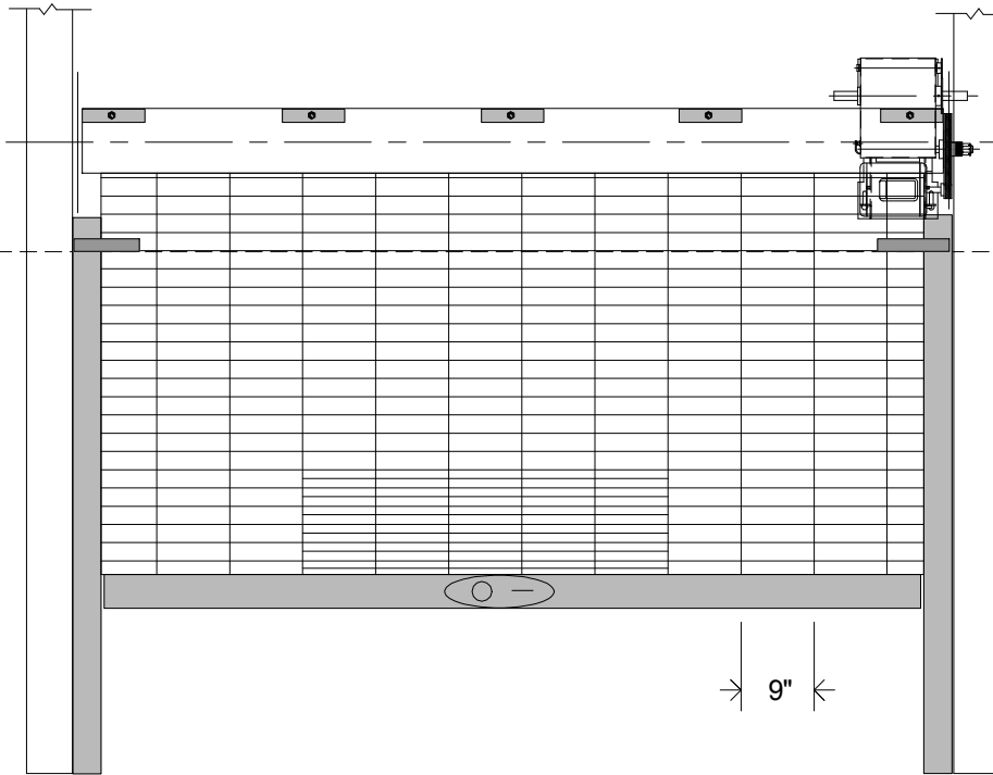
Coil Side Elevation Detail
