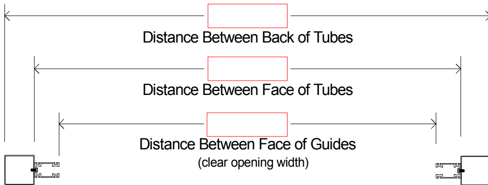
Plan View - Coil Side
