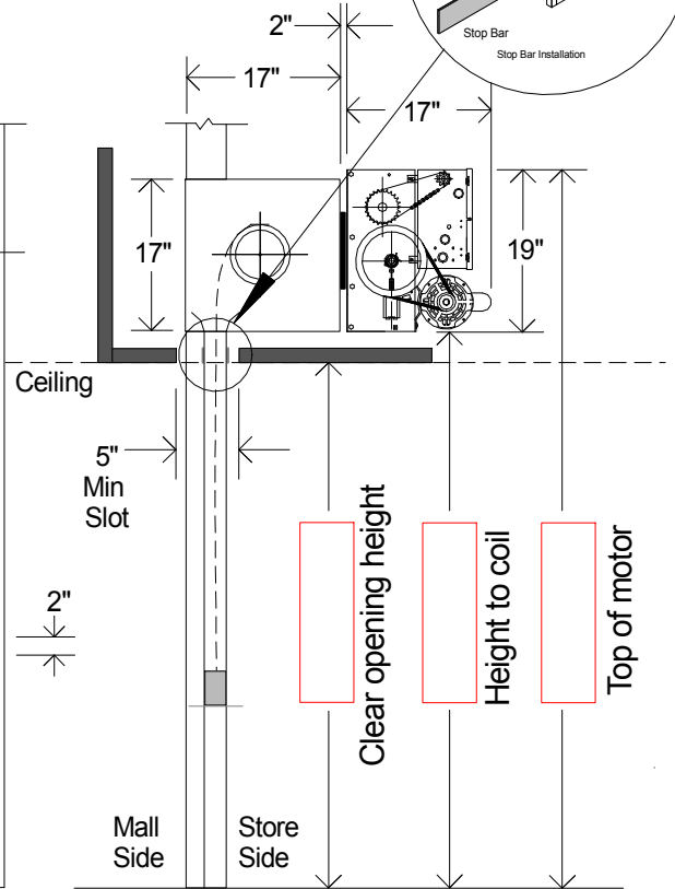
Storefront Section
