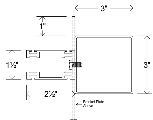
Storefront Section
